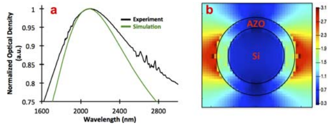
Figure 3 (a) FDTD simulations showing a comparison of the experimental (black) and simulated (green) extinction spectra for a SiNP ( D = 200 nm) coated with a 50 nm thick, 1 : 15 Al 2 O 3 : ZnO cycle ratio AZO film. (b) Cross-section of an AZO-coated SiNP nanopillar while excited with linearly polarized light at peak resonance (2085 nm).
